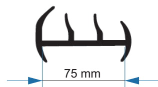
Borracha RD Frigorifica 99.00.133
