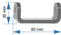
Cavalete 10.02.012
