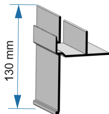
Saia 130 50.01.168
